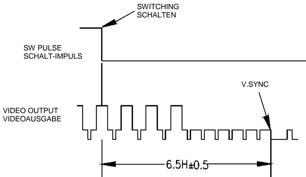
Playback phase adjustment Playback-phaseneinstellung Fig.49. Abb.49.
